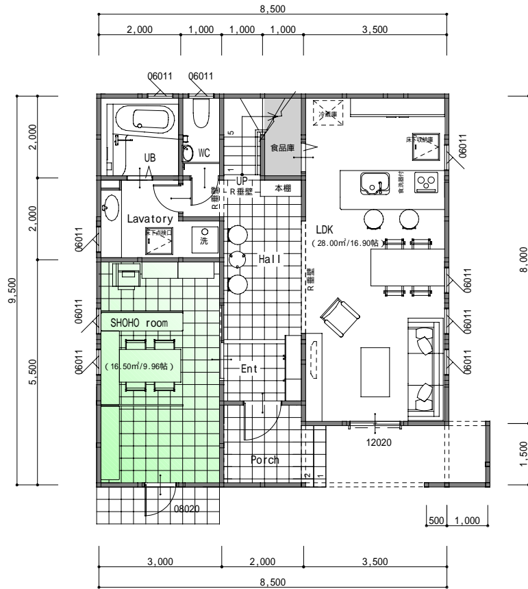
1F Plan
