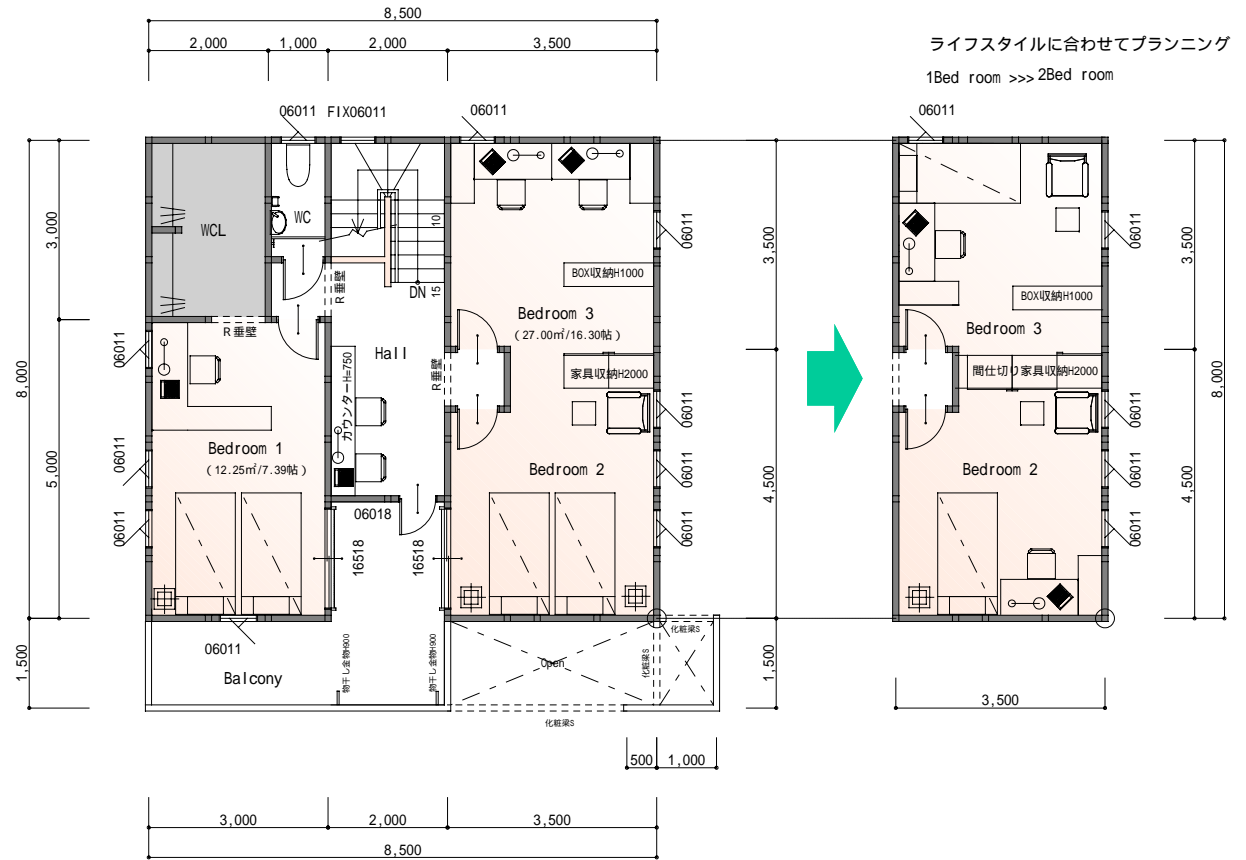
2F Plan
